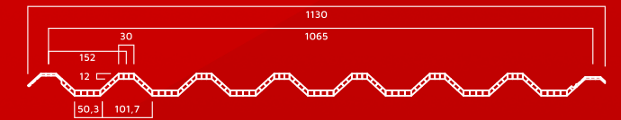
Drawing - Twin Wall RF 1065
