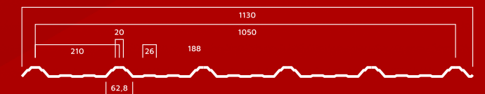
Drawing - Single Wall RF 1050
